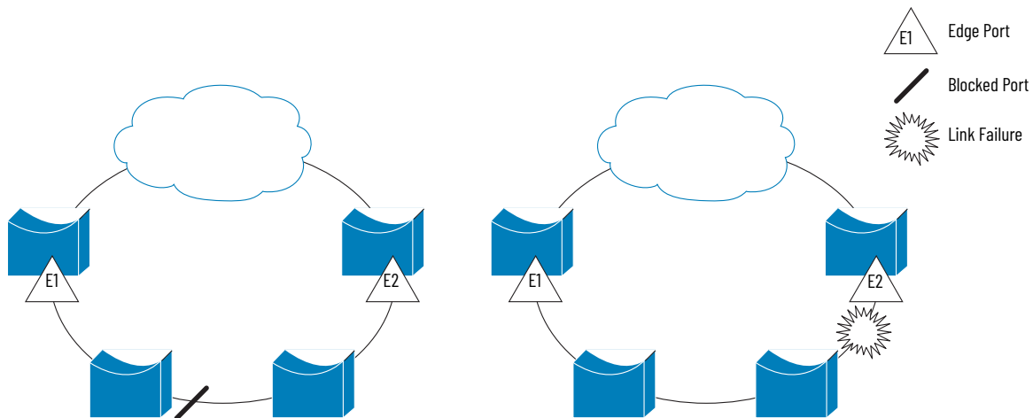
Figure 33 - Open Segment Example
