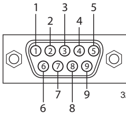
Figure 73 - DB-9 Connector Pinout
