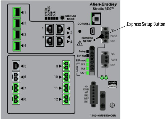
Stratix 5400 Switch
