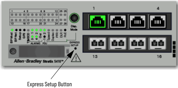
Stratix 5410 Switch
