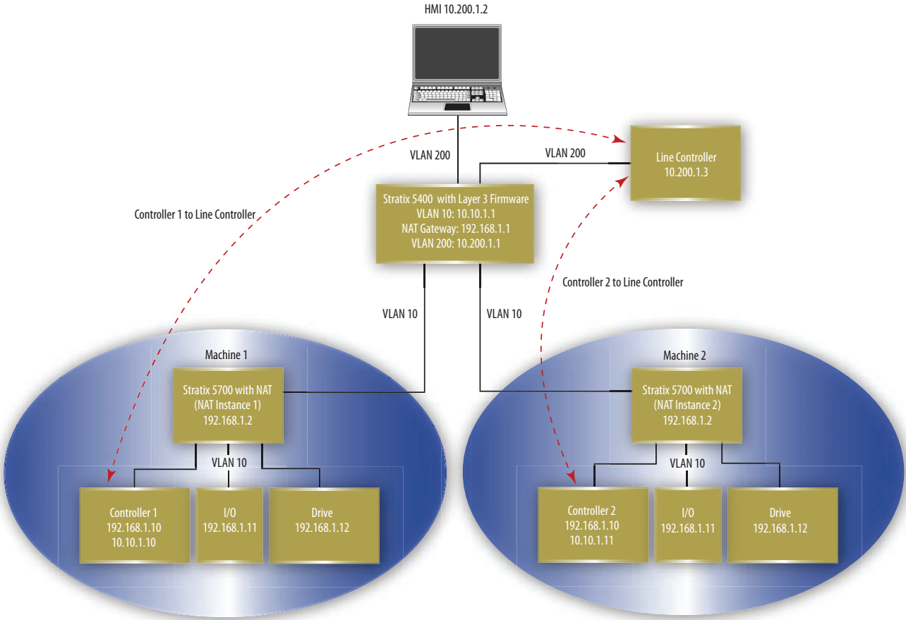
Figure 16 - Layer 3 Example with NAT in Stratix 5700 Switch
