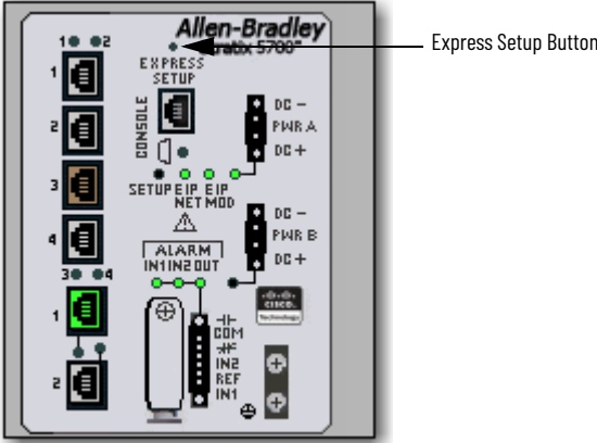
Stratix 5700 Switch
