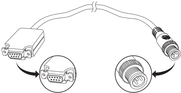
Figure 71 - M12-to-DB-9 Cable
