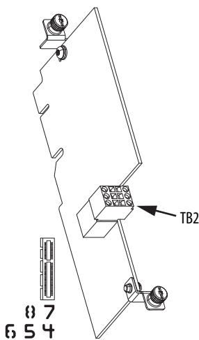
20-750-S Safe Torque Off Option Module
