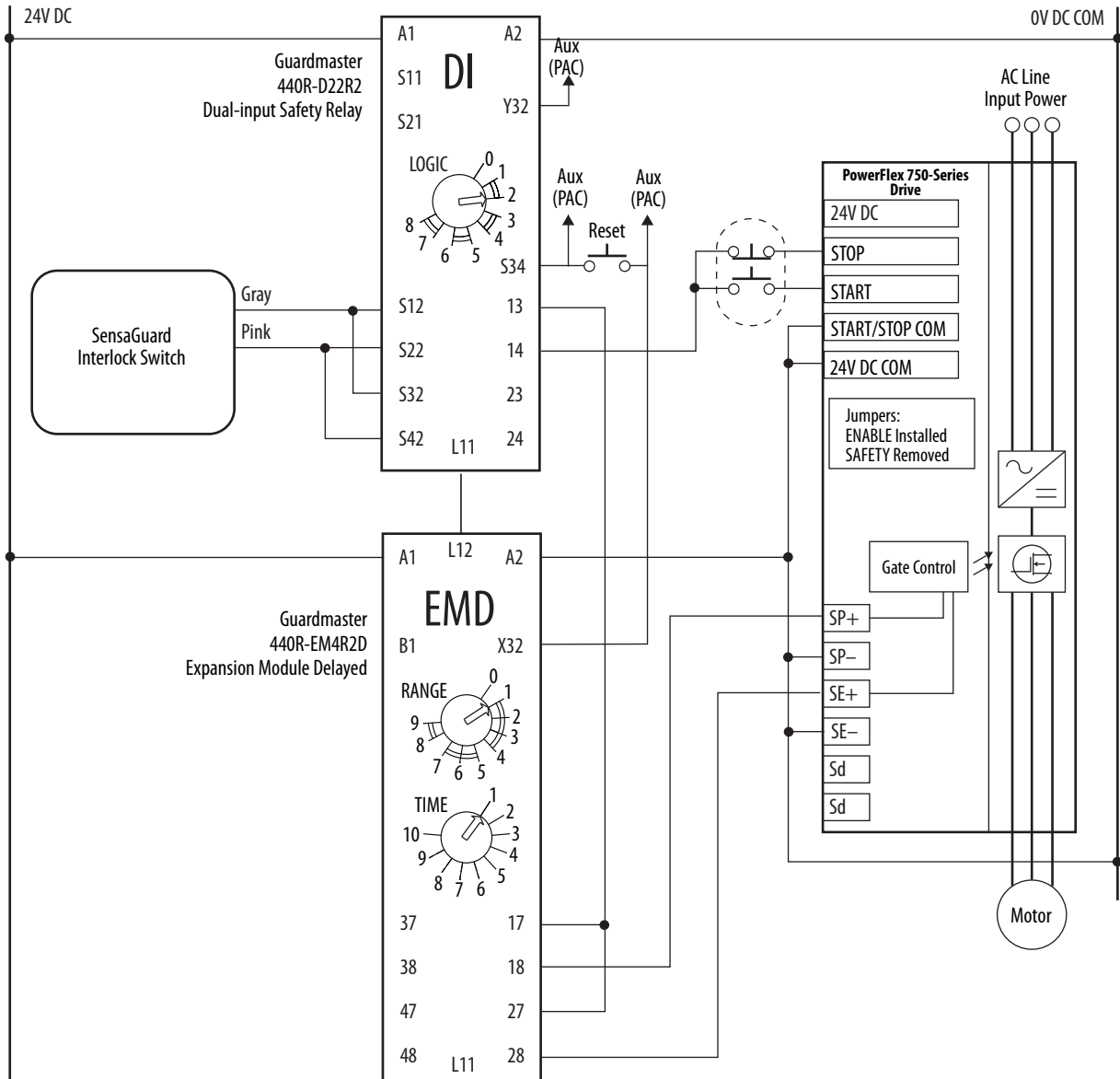
Figure 8 - Stop Category 1
