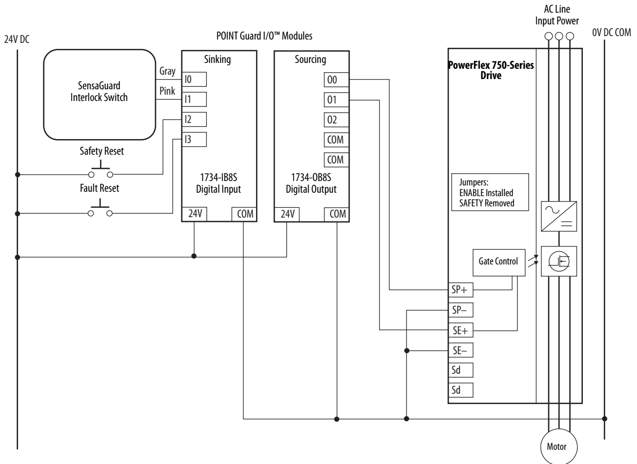
Figure 9 - Stop Category 0
