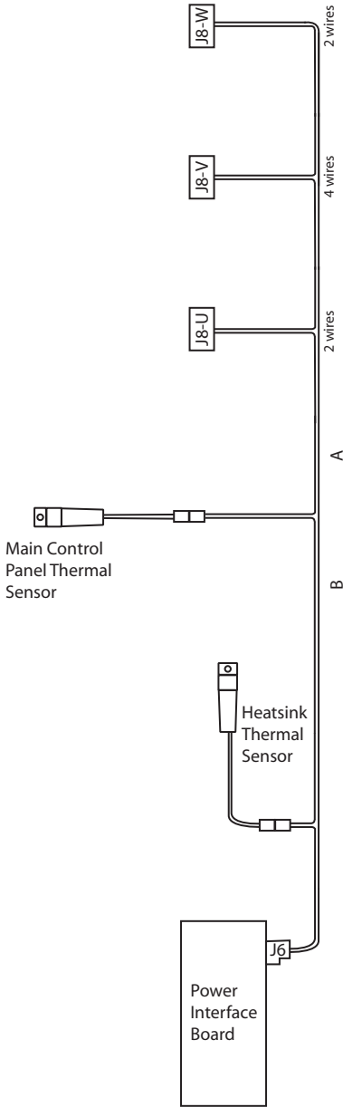
Thermal Sensor wiring for both drives
