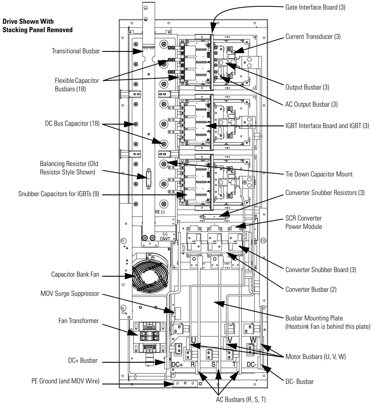
Figure 1 - Frame 8 AC Drive Components
