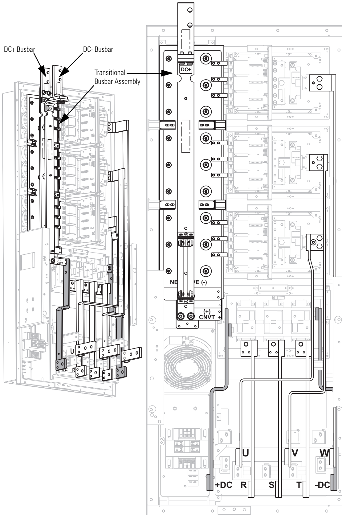
Figure 3 - Frame 8 Busbars (AC Drive shown)
