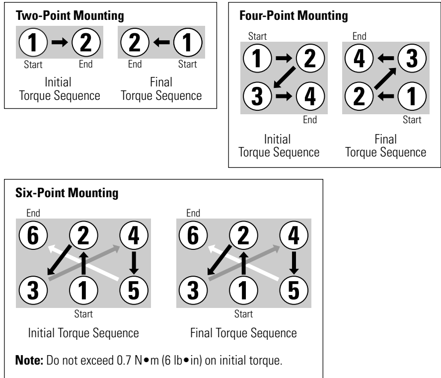
Figure 6 - Various-point Mounting
