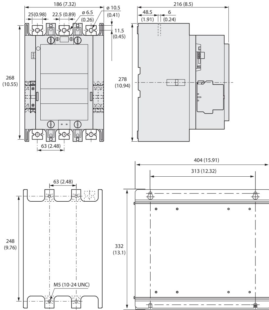
Figure 88 - 100-E400, 100-E460 Contactors with PLC Input
