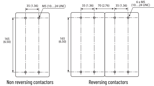
Figure 84 - 100-E265...100-E370 Contactors
