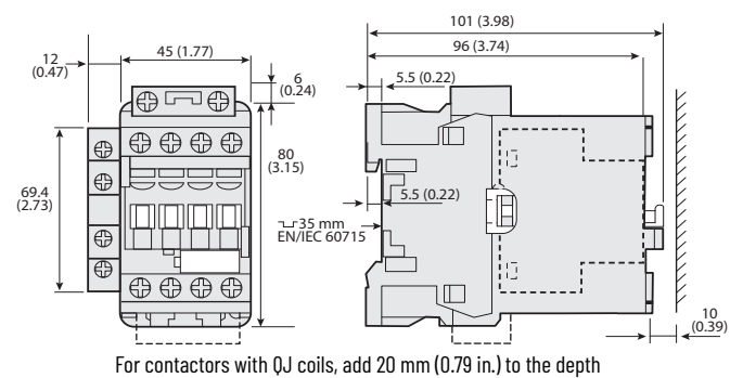
Figure 50 - 100-E26...100-E38 4-Pole Contactors with Standard Coils and Side-mounted Auxiliary Contact
