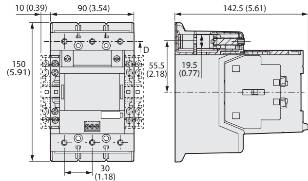
Figure 78 - 104-E116E..., 104-E146E... Reversing Contactors with Cat. No. 100-EM... Mechanical Interlock
