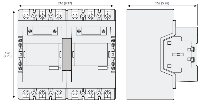
Figure 86 - 104-E265...104-E370 Reversing Contactors with Cat. No. 100-EM... Mechanical Interlock
