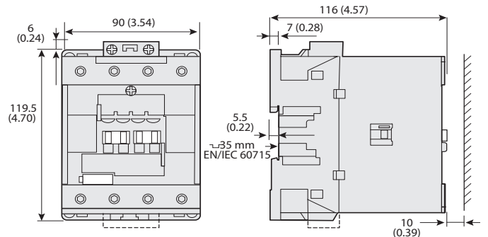
Figure 71 - 100-E80 4-Pole Contactors
