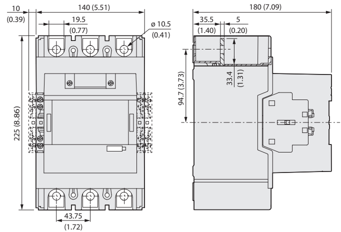
Figure 84 - 100-E265...100-E370 Contactors
