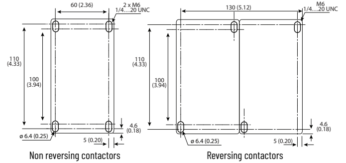
Figure 71 - 100-E80 4-Pole Contactors
