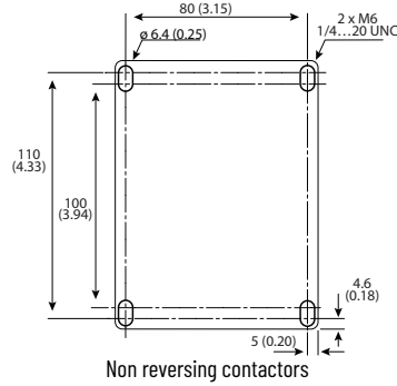
Figure 74 - Drilling Template for 80 A 4-Pole Contactors
