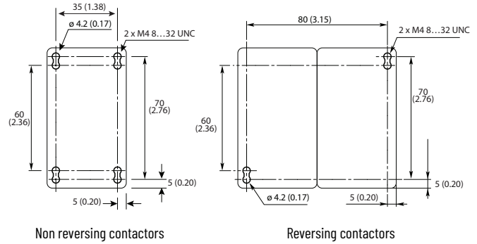
Figure 62 - 100-E40...100-E52 4-Pole Contactors
