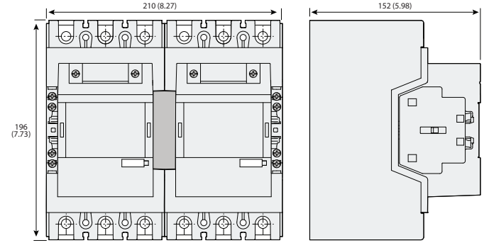
Figure 83 - Drilling Template for 190...205 A 3-Pole Contactors
