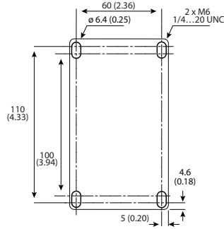
Figure 65 - Drilling Template for 40...52 A 4-Pole Contactors
