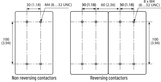
Figure 80 - 100-E190, 100-E205 Contactors
