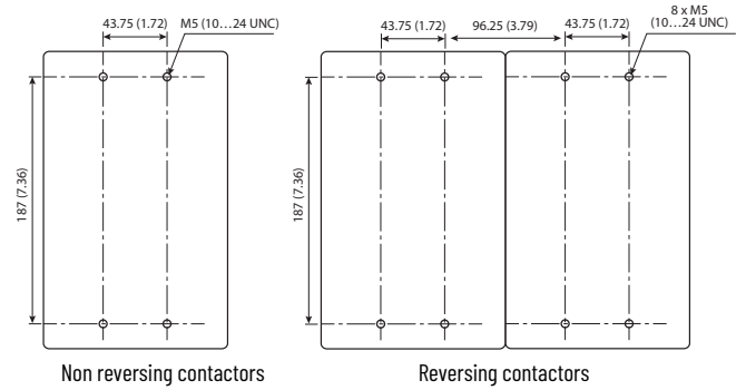
Figure 87 - Drilling Template for 265...370 A 3-Pole Contactors
