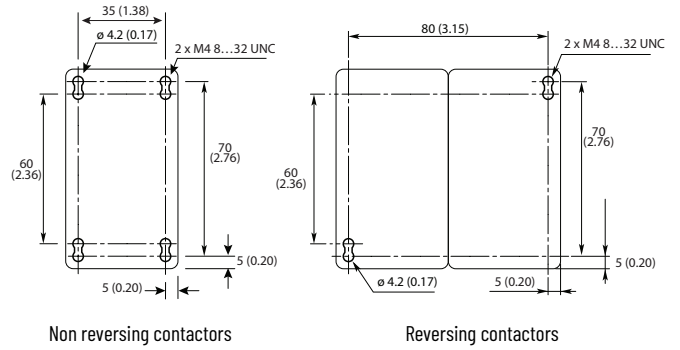
Figure 56 - Drilling Template for 26...38 A Contactors
