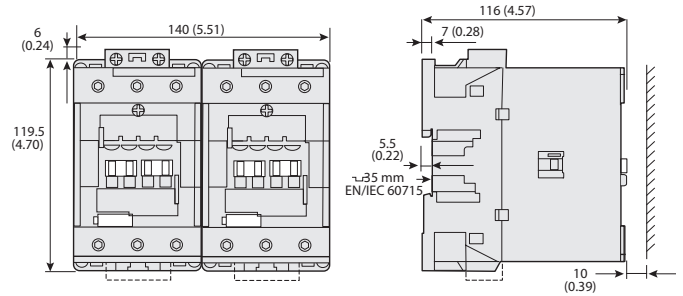
Figure 70 - Drilling Template for 80...96 A 3-Pole Contactors
