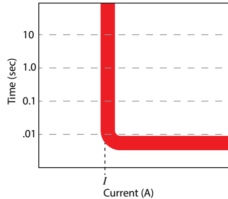
Example of magnetic time vs. current curve.
