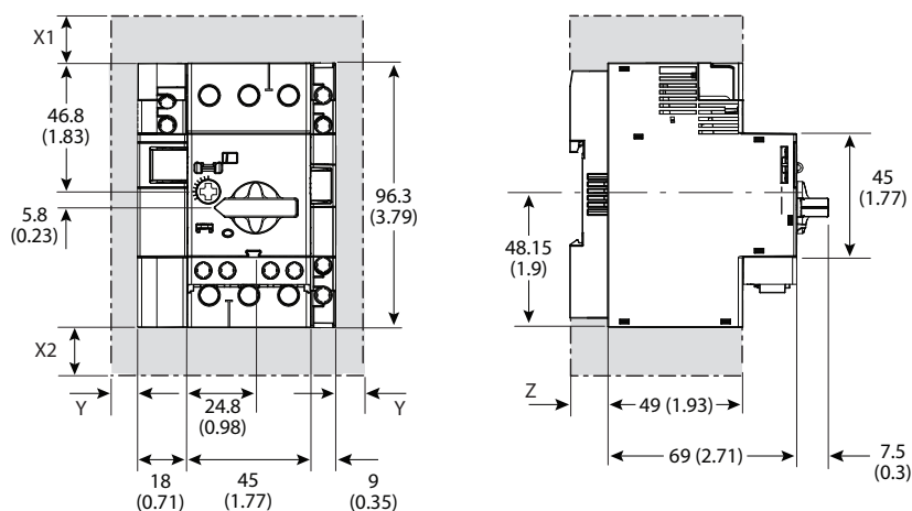
Figure 12 - Spacing Requirements
