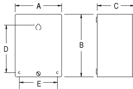
Type 1 Enclosure
