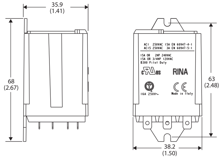
700-HD Relay
