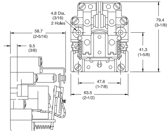
700-HG Relay
