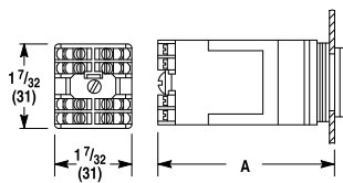
Screw Terminals with Pressure Plate Contact Block (Typical View) (1)
