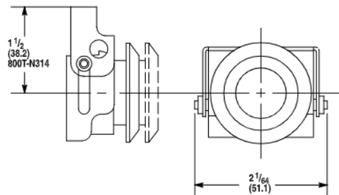
Push-pull/Twist Padlocking Attachment
