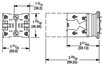
Stackable Sealed Switch Block 1.58 (40.1) Deep
