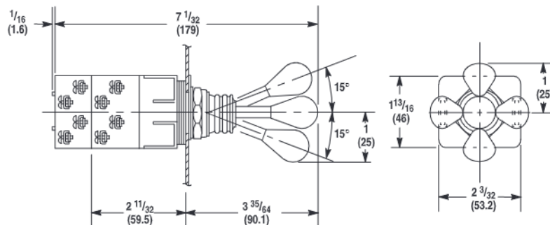
2-3-4 Way Switch
